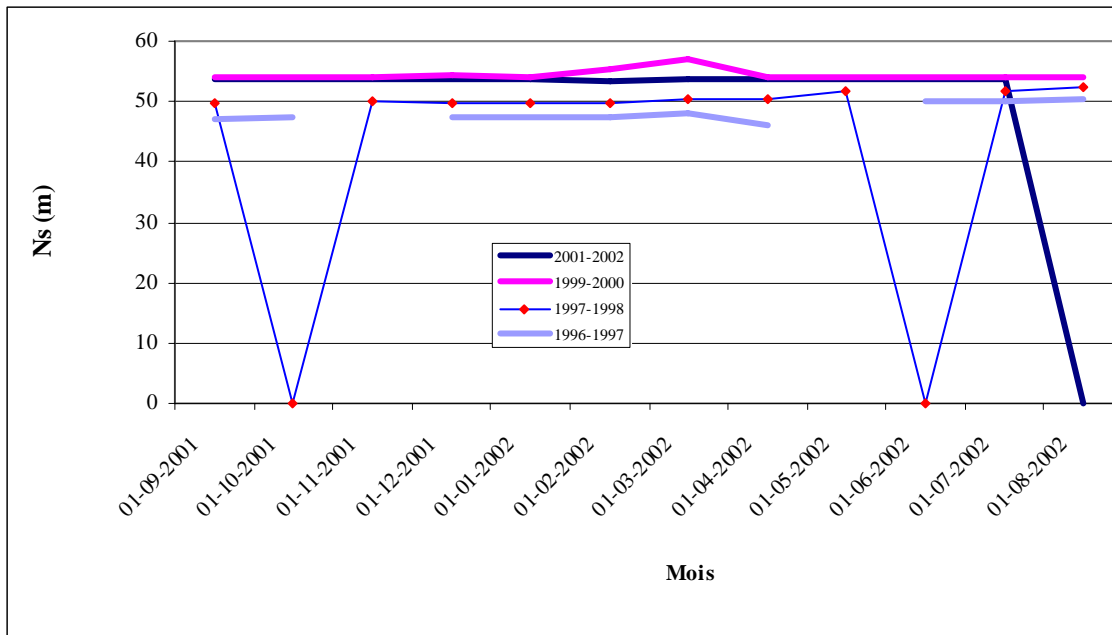
Figure 10. Comparison of the NS of the Well witness W212-0092 of 1996 to 2002
