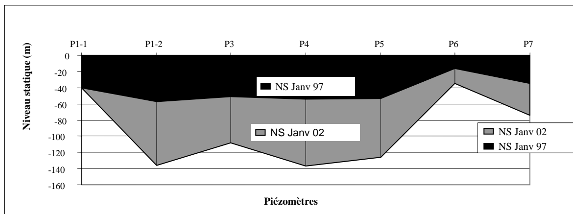
Figure 6. Folding back in the piezometer s : Janv 1997 – Janv 2002
