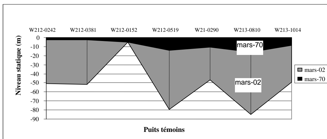
Figure 5. Folding back in the wells: March 1970 – March 2002
