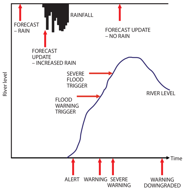
Figure 8.4. Flood forecasting and warning schematic
