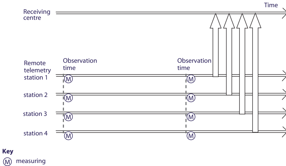
Figure . . Diagram of the batch reporting method
