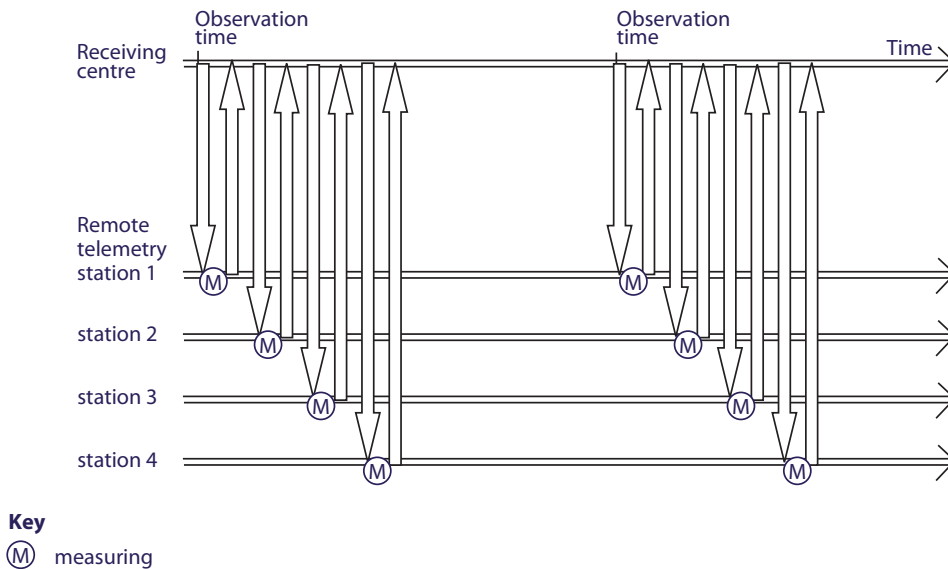
Figure .4. Diagram of on-demand polling
