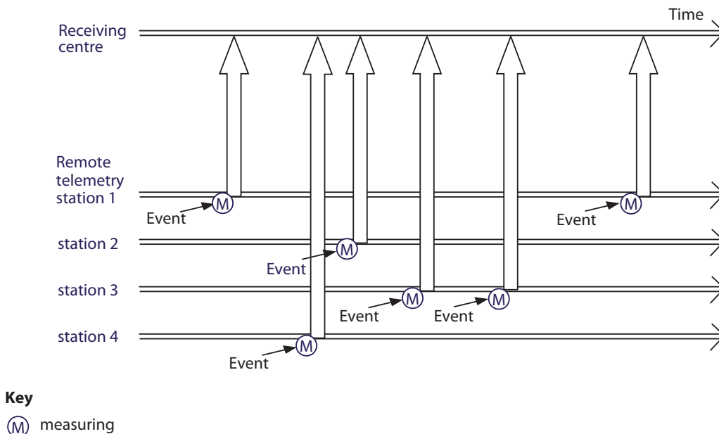
Figure .7. Diagram of the event reporting method
