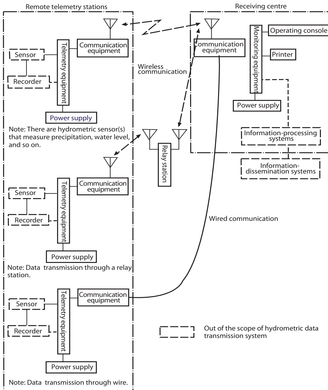
Figure .1. Conceptual configuration of an HDTS
