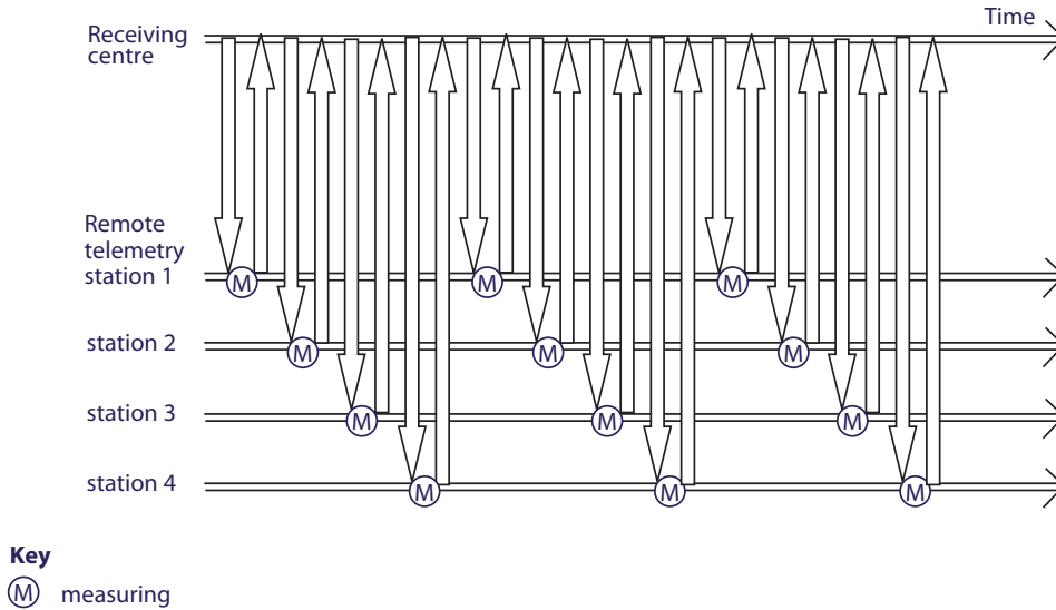
Figure .3. Diagram of cyclic polling
