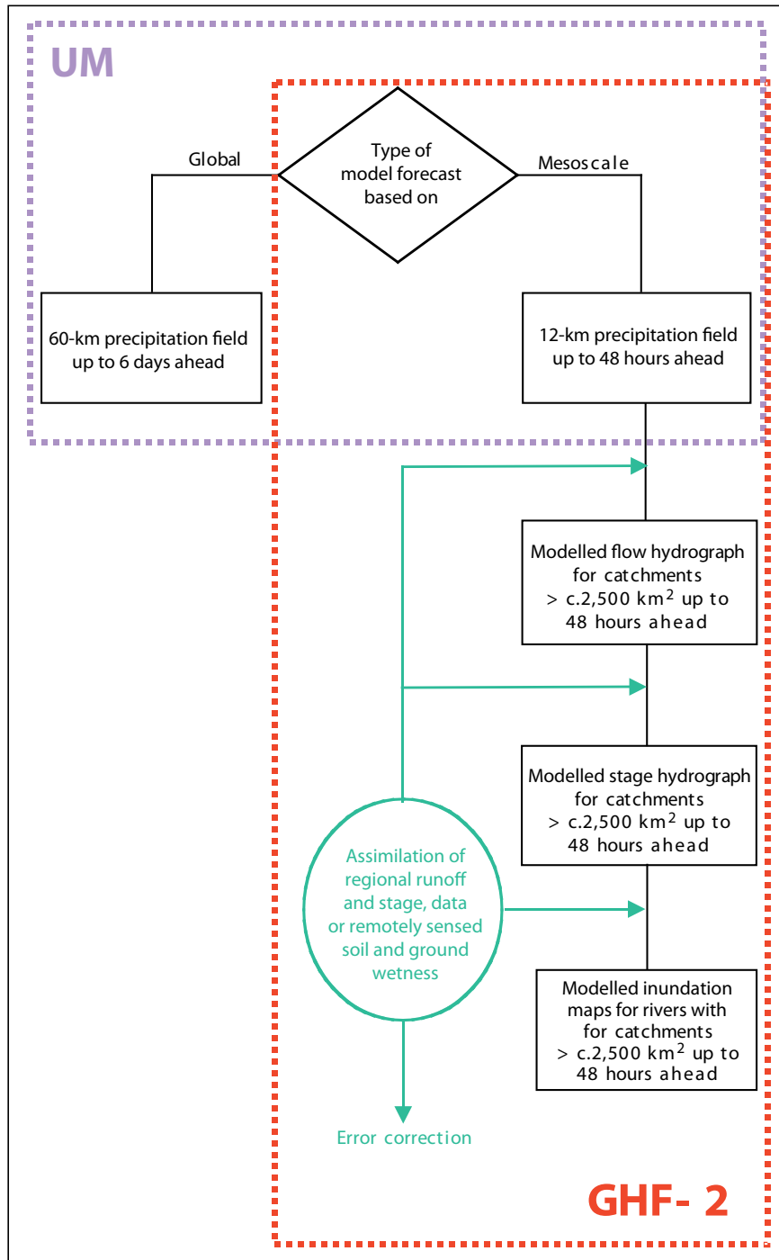
Figure 4.3. F based on mesoscale model fields ( F-2)
