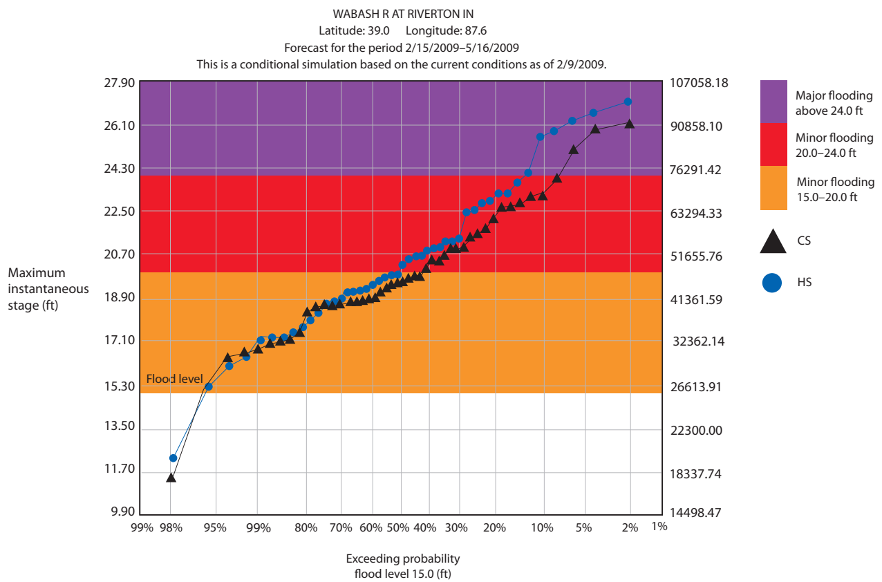
Figure 7.7. A PS flood forecast stages probability hydrograph for the Wabash River with PF input. The CS (conditional simulation) line indicates the chances of the river exceeding given levels based on current conditions. The S (historical simulation) line indicates the chances of the river exceeding given levels based on the total range of past levels.
